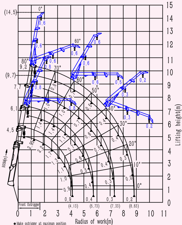
SPT299 Load Chart With Fly Jib
