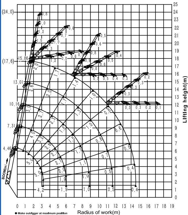
S11 Load Chart With Fly Jib
