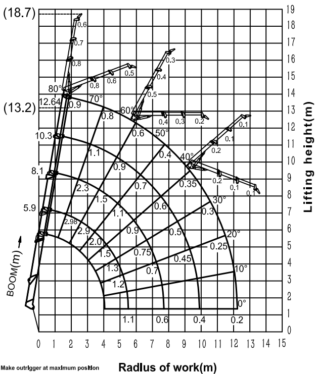
SPT399-Load Chart
