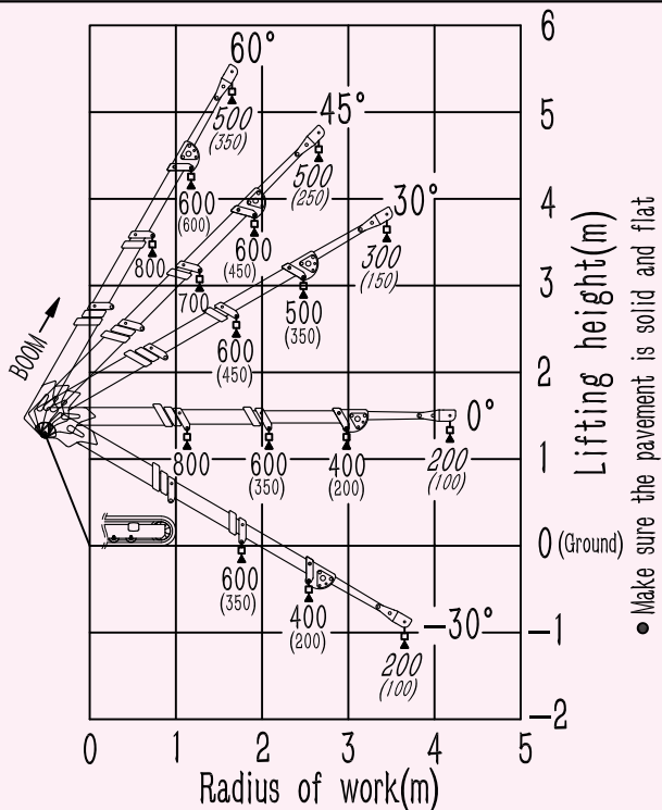
SG80 Load Chart With Fly Jib
